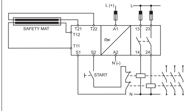
NST02C...SA, NST02C...SC
