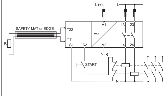
NSE02C...SA, NSE02C...SC
