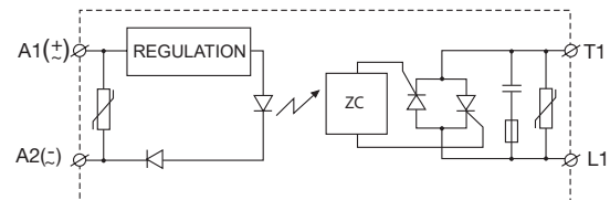
Tension CA
