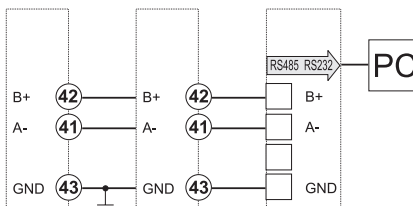
Fig. 29 Puerto RS485
