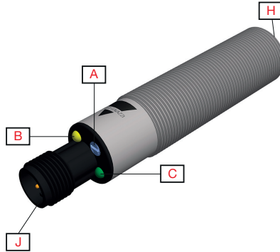
Fig. 2 CA18 Conector
