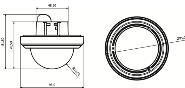
Fig. 2 Built-in version
