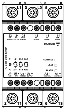
RGC2..75..DFM RGC3..65..DFM
